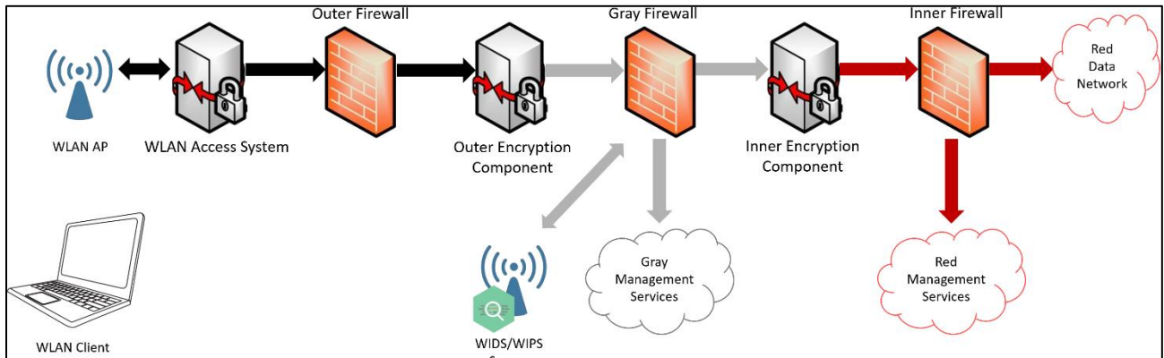
Figure 4: MA with Overlay WIDS/WIPS in Gray Management
