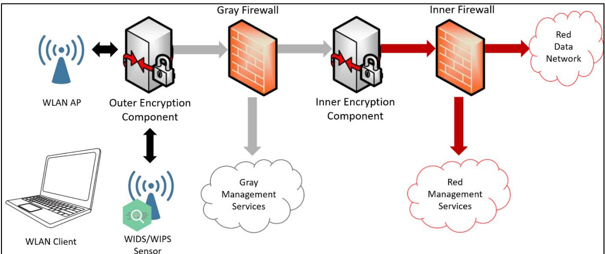
Figure 3: Campus WLAN CP Black Integrated WIDS
