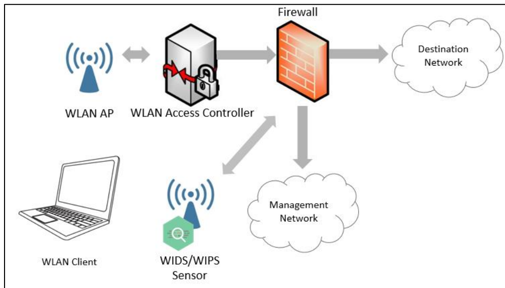
Figure 17: Overlay WIDS/WIPS
