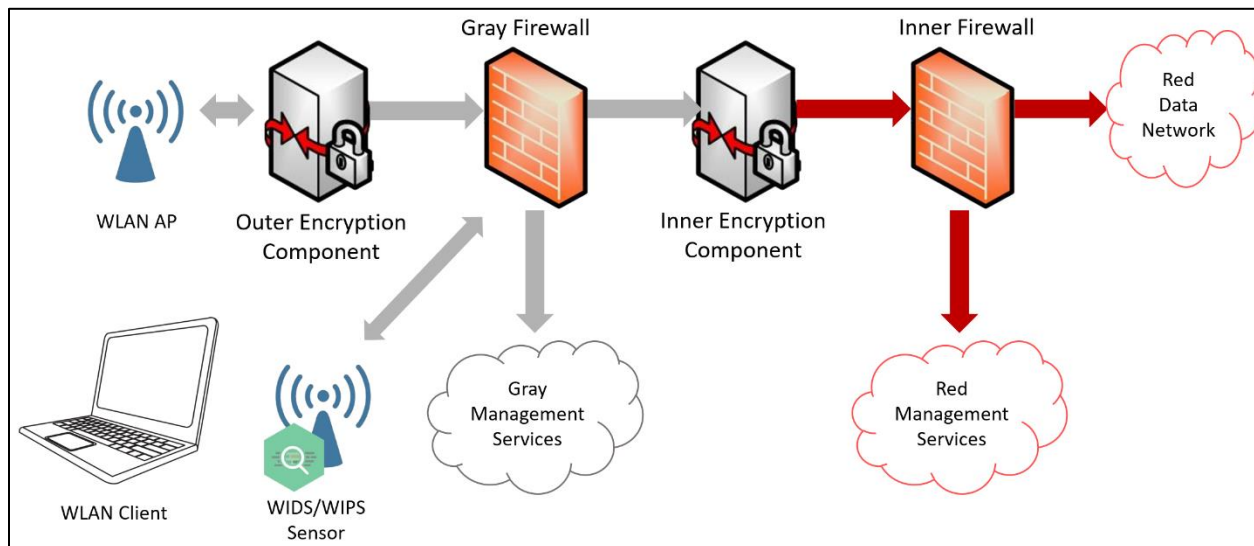
Figure 6: WLAN with Overlay WIDS/WIPS in Gray Management
