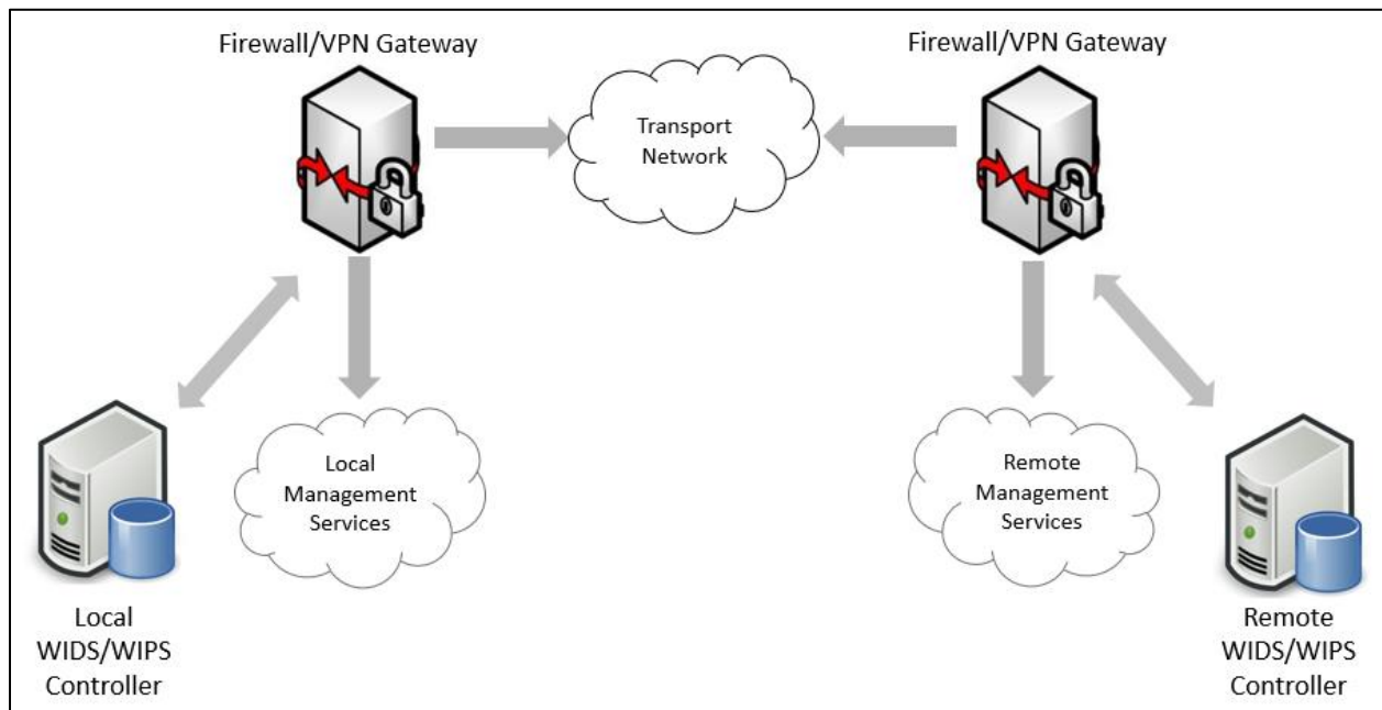
Figure 19: WIDS/WIPS Remote Systems
