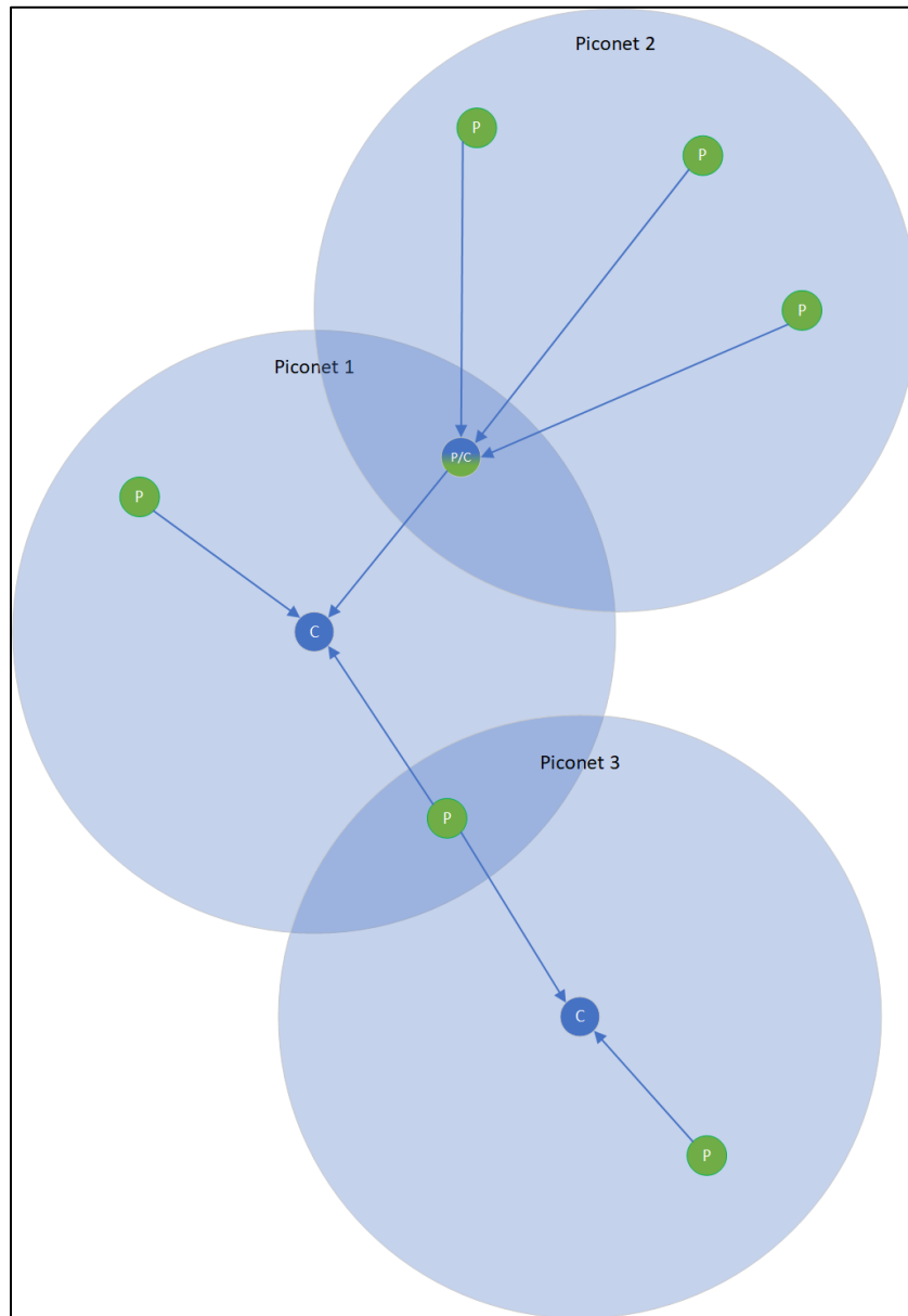
Figure 15: Bluetooth Scatternet
