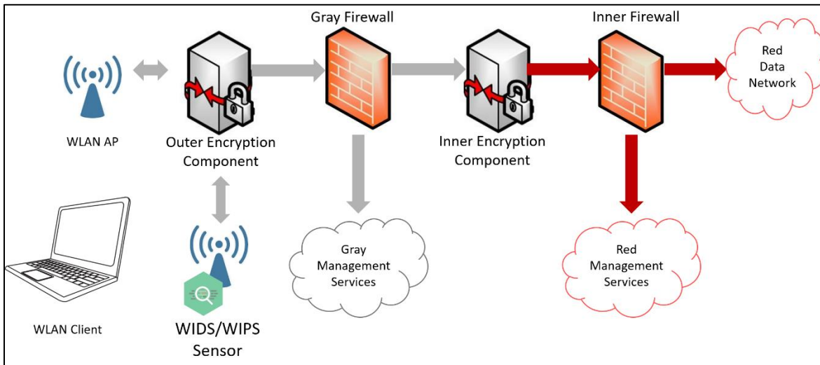
Figure 1. WLAN with Integrated Gray WIDS/WIPS
