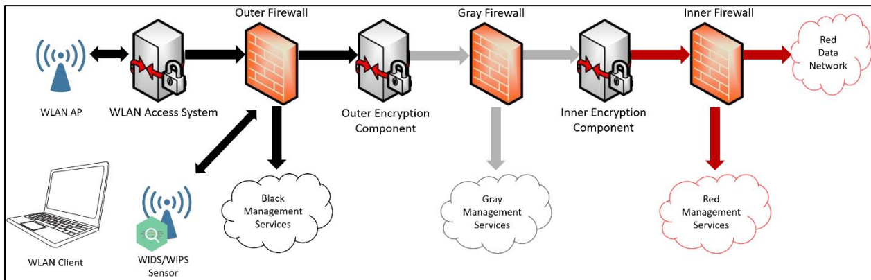
Figure 5: MA with Overlay WIDS/WIPS in Black Management
