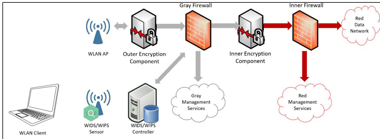
Figure 8: WLAN with Separate WIDS/WIPS Networks
