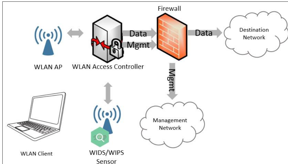
Figure 16: Integrated WIDS/WIPS
